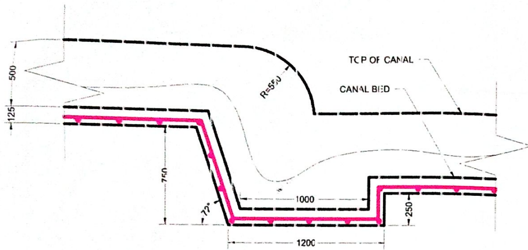
PLAN OF CANAL DROP SCALE 1:20
