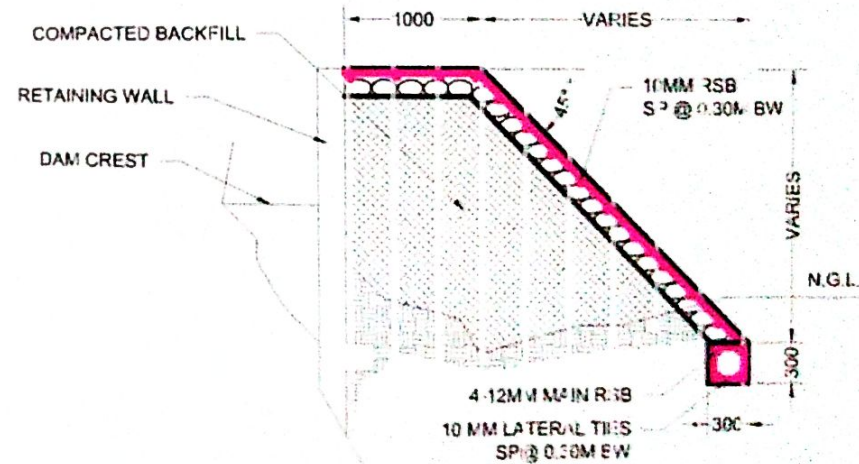
DETAIL D SCALE 1:40
