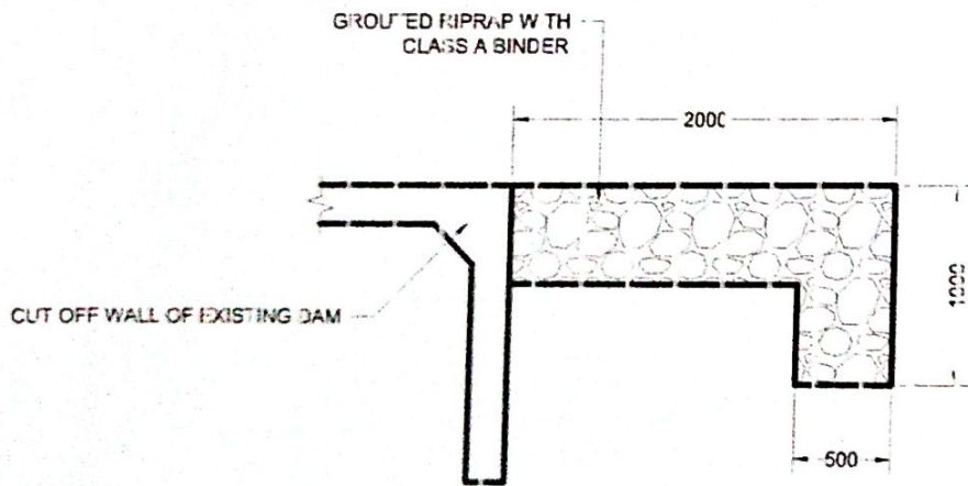
C GROUTED RIPRAP SCALE 1:16
