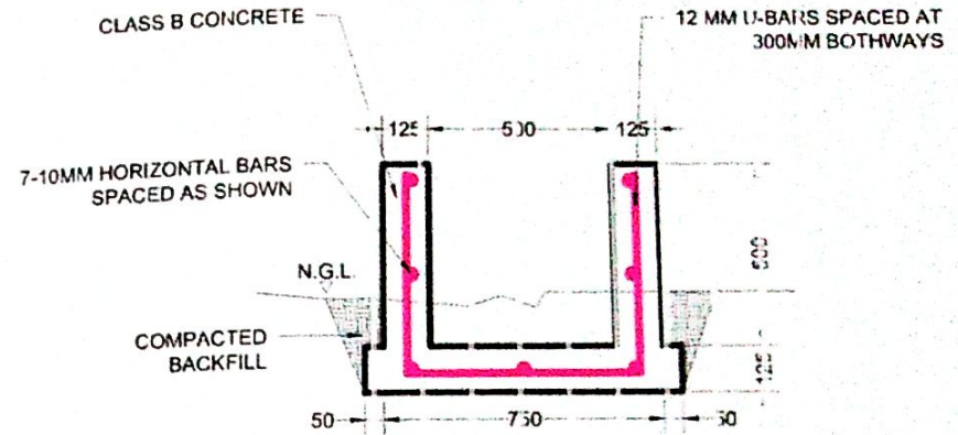
PLAN OF CANAL SCALE 1:6
