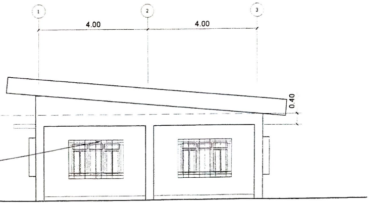
2 A 2 LEFT SIDE ELEVATION SCALE 1:100 M
