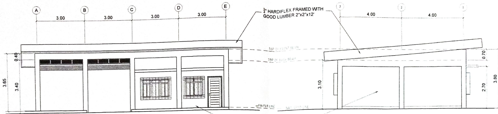
1 A 2 FRONT ELEVATION SCALE 1:100 M
