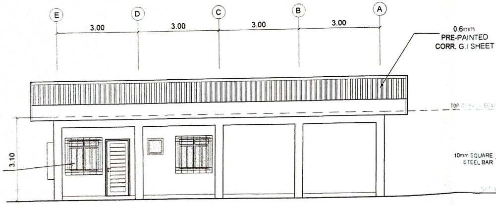
1 A 2 FRONT ELEVATION SCALE 1:100 M
