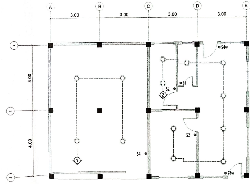
3 A 3 LIGHTING LAYOUT SCALE 1:100 M
