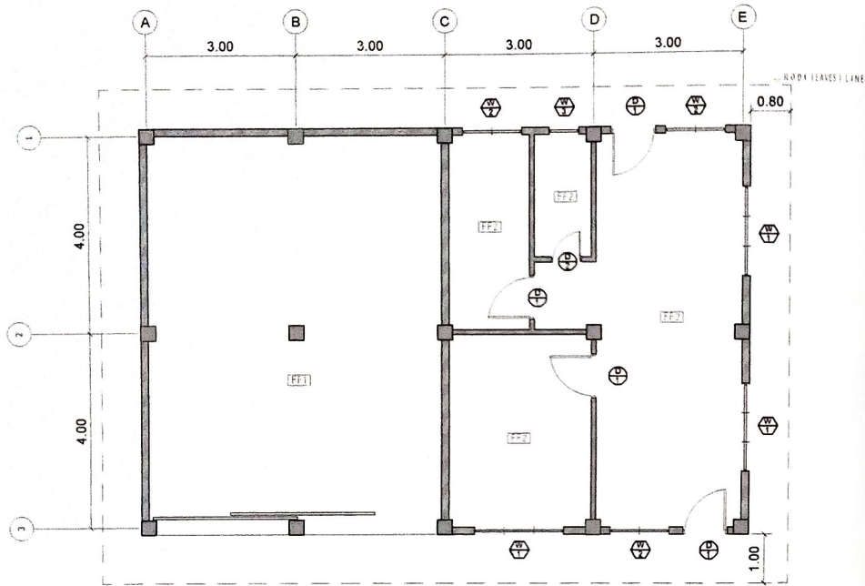
1 A 1 FLOOR PLAN SCALE 1:100 M
