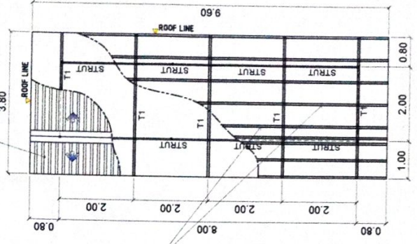
3 ROOF FRAMING PLAN SCALE 1:100 MTS
