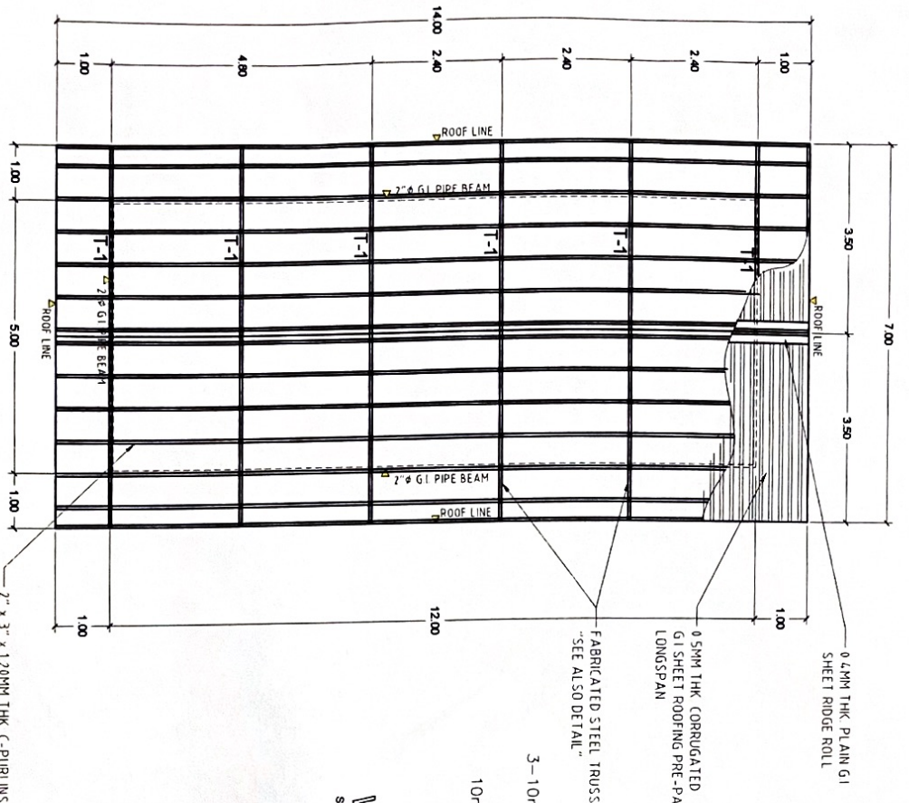
ROOF FRAMING LAYOUT SCALE 1:100M
