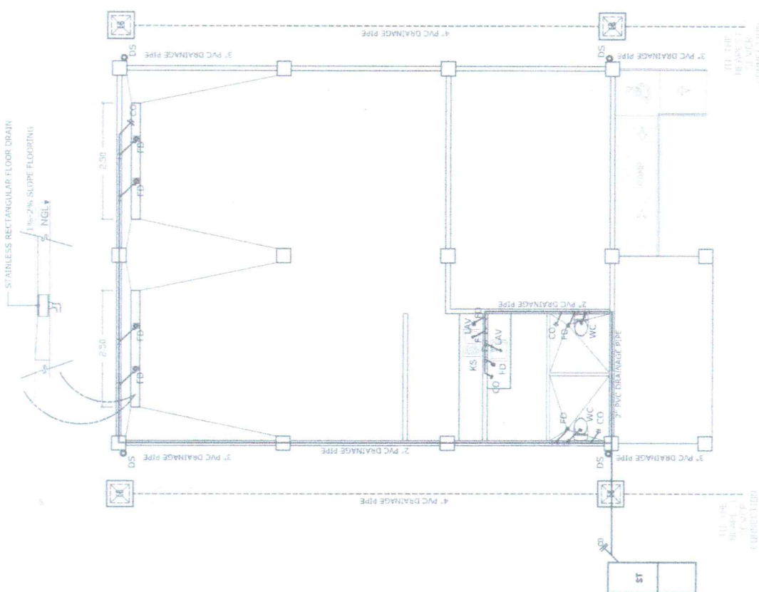
SEWER LINE LAYOUT
