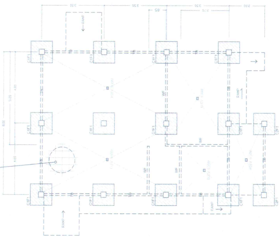
FOUNDATION LAYOUT SCALE 1:50 M
