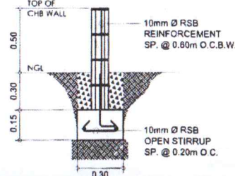
CHB WALL FOOTING DETAIL SCALE 1:25 M.
