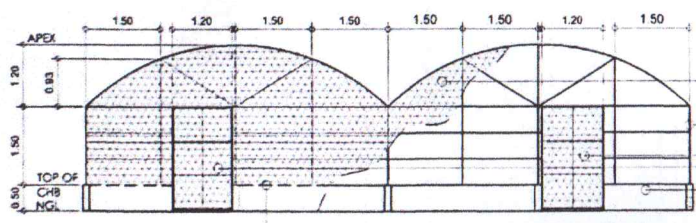
FRONT ELEVATION SCALE 1:100 M.
