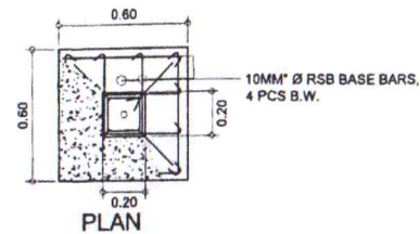
CONCRETE PEDESTAL DETAIL SCALE 1:25 M. = 21 SETS
