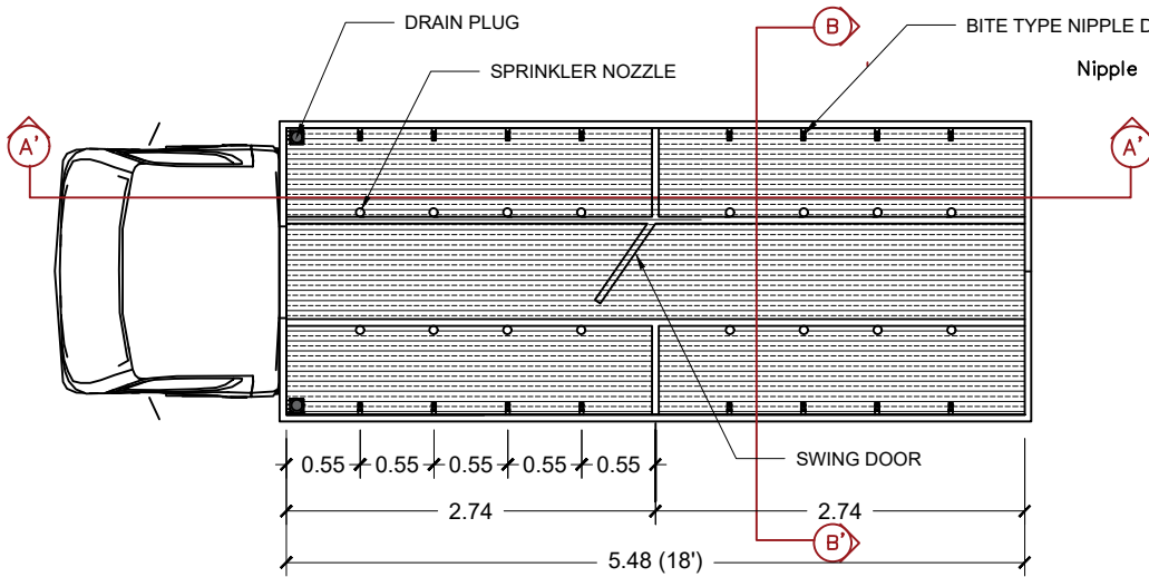
SET-UP FOR FINISHER @ 24 HEADS/LAYER Scale: NTS
