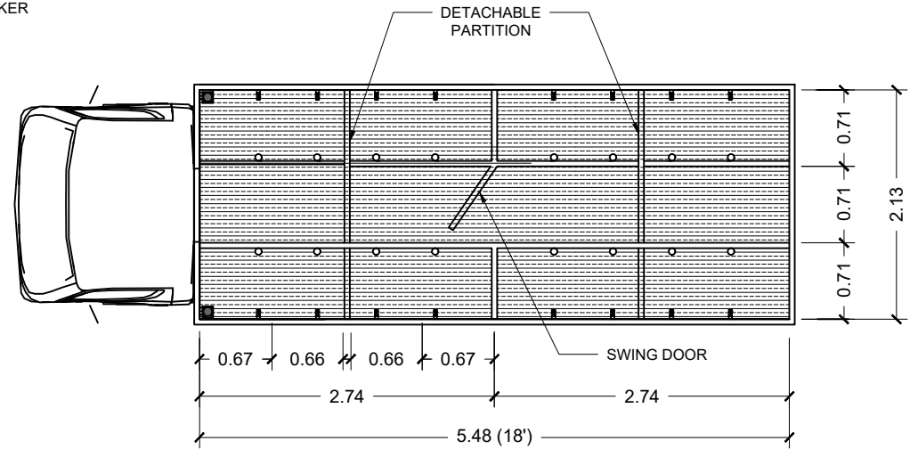
SET-UP FOR WEANER (20kg) @ 70 HEADS/LAYER Scale: NTS
