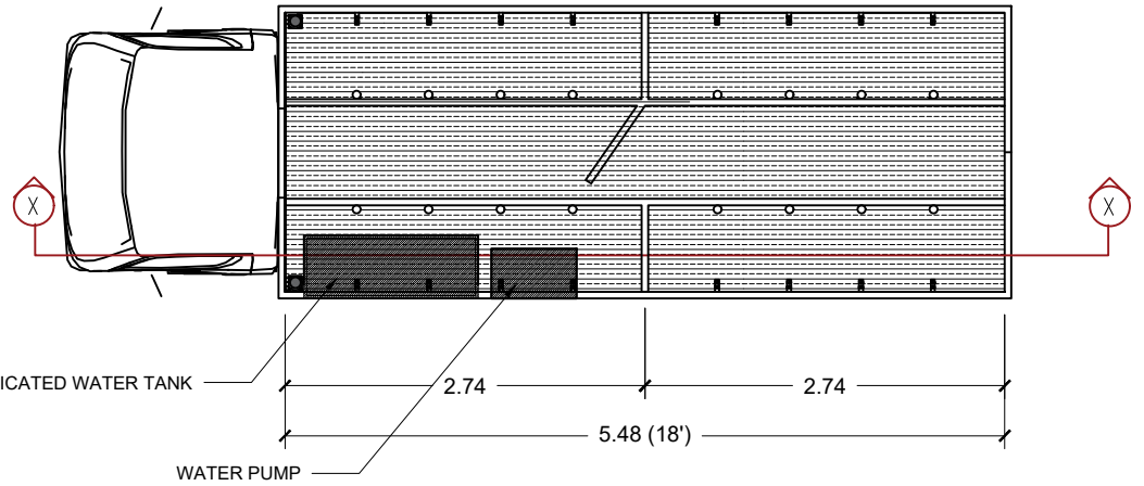
SET-UP FOR WATER LINE @ TOP VIEW Scale: NTS
