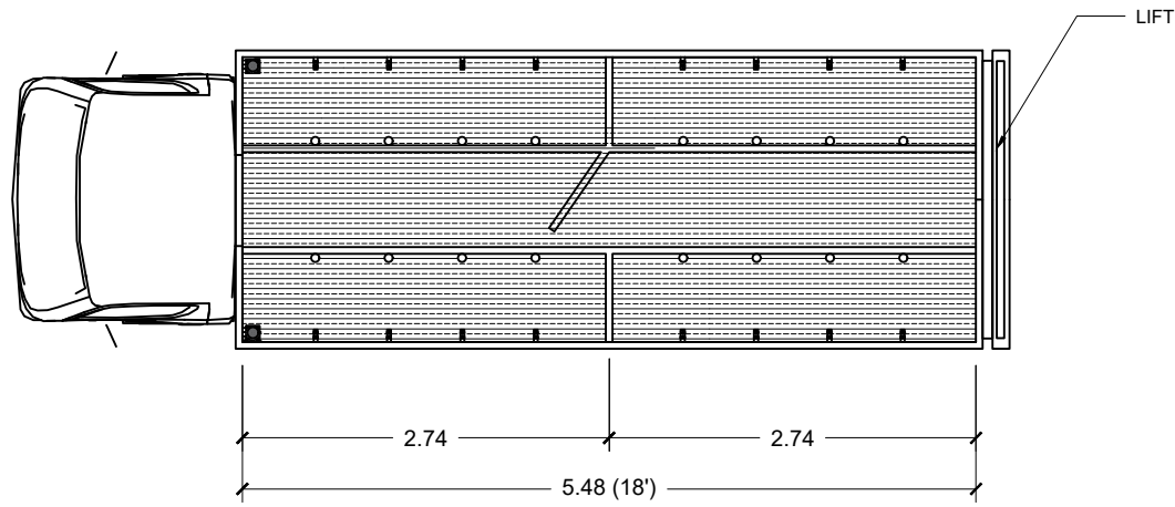
LOWER/UPPER DECK FLOOR PLAN Scale: NTS
