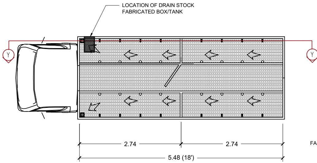
SET-UP FOR DRAIN LINE @ TOP VIEW Scale: NTS
