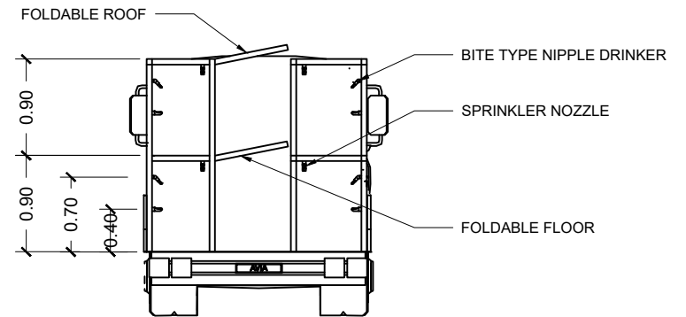
CROSS SECTION THRU "B-B" Scale: NTS
