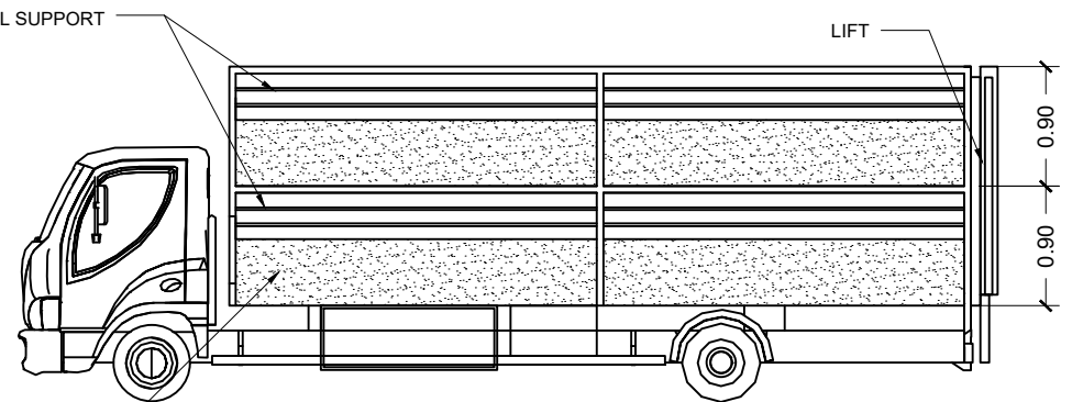
RIGHT SIDE ELEVATION Scale: NTS
