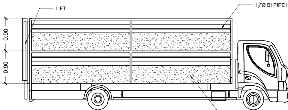
LEFT SIDE ELEVATION Scale: NTS
