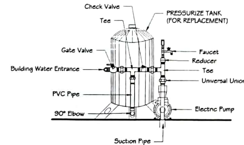
HYDRO-PNEUMATIC SYSTEM
