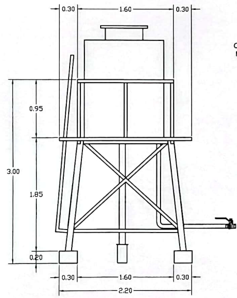
SIDE ELEVATION SCALE 1: 40 MTS.
