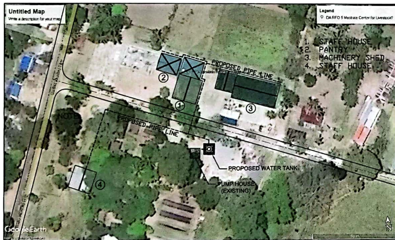
PIPE LINE LAYOUT
