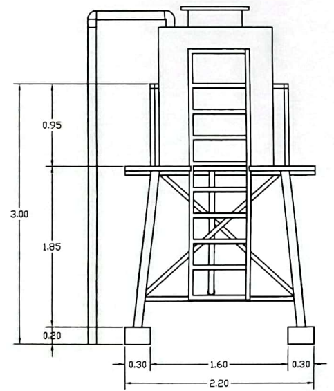
FRONT ELEVATION SCALE 1: 40 MTS.
