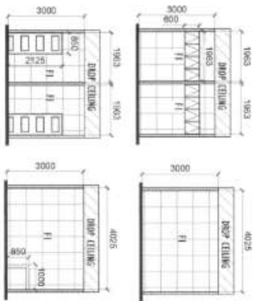
SECTION FOR WALL TILES SCALE: 1:100
