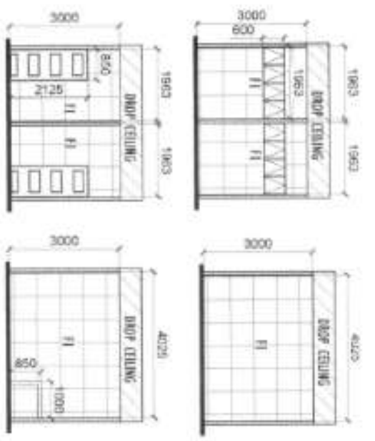
A SECTION FOR WALL TILES SCALE: 1:100
