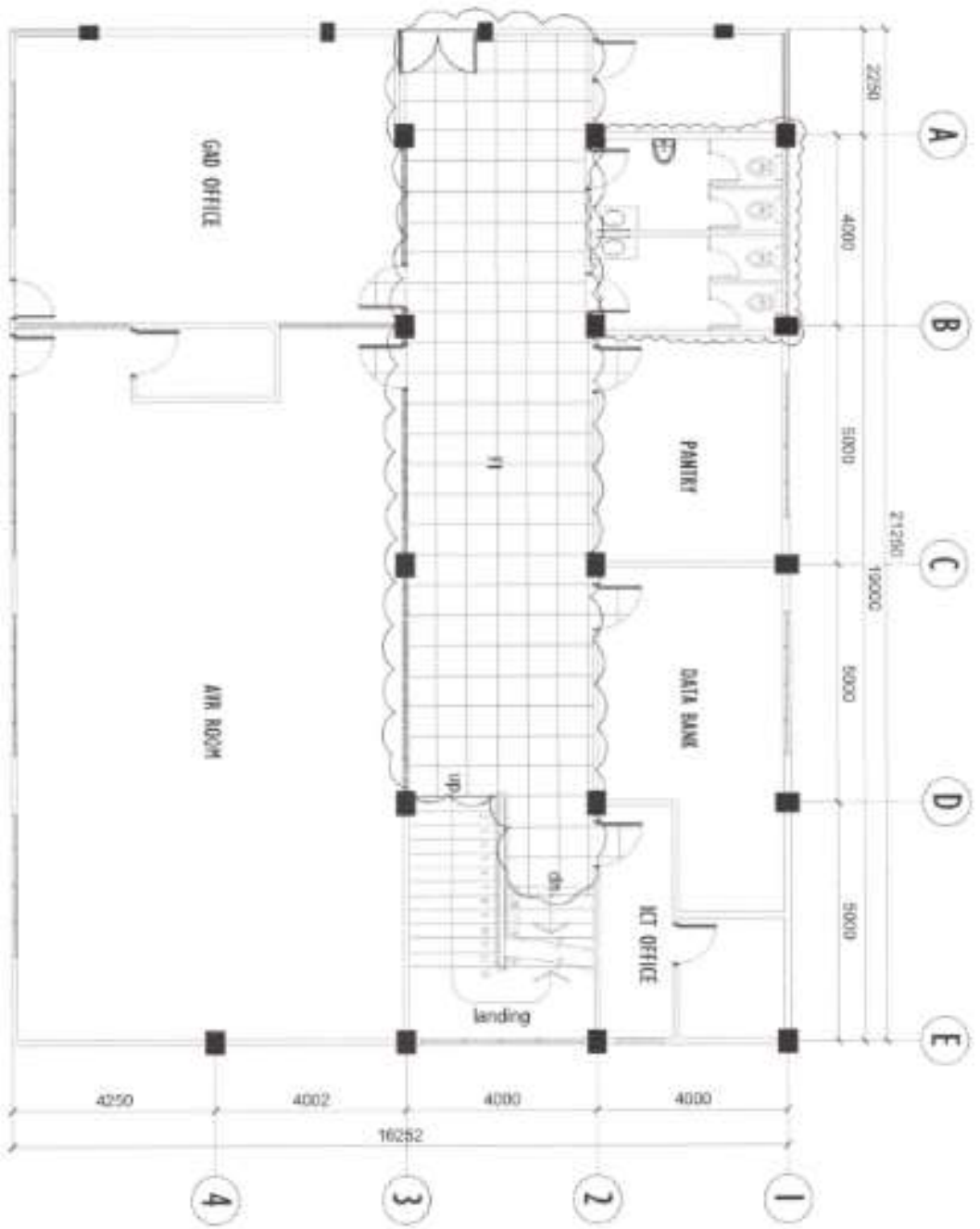
THIRD FLOOR PLAN SCALE: 1:100
